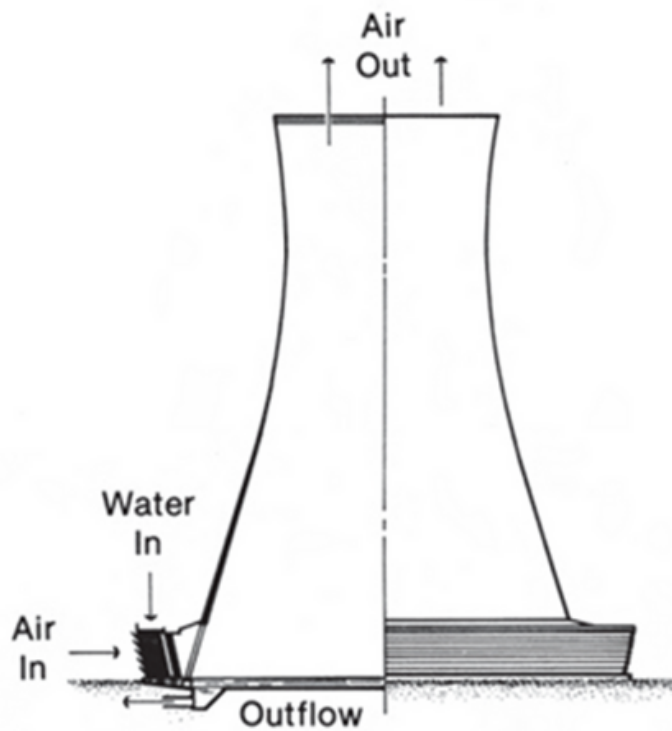
CROSSFLOW NATURAL DRAFT TOWER
