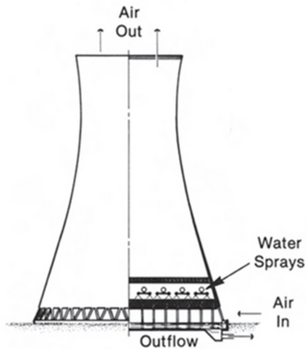
COUNTERFLOW NATURAL DRAFT TOWER
